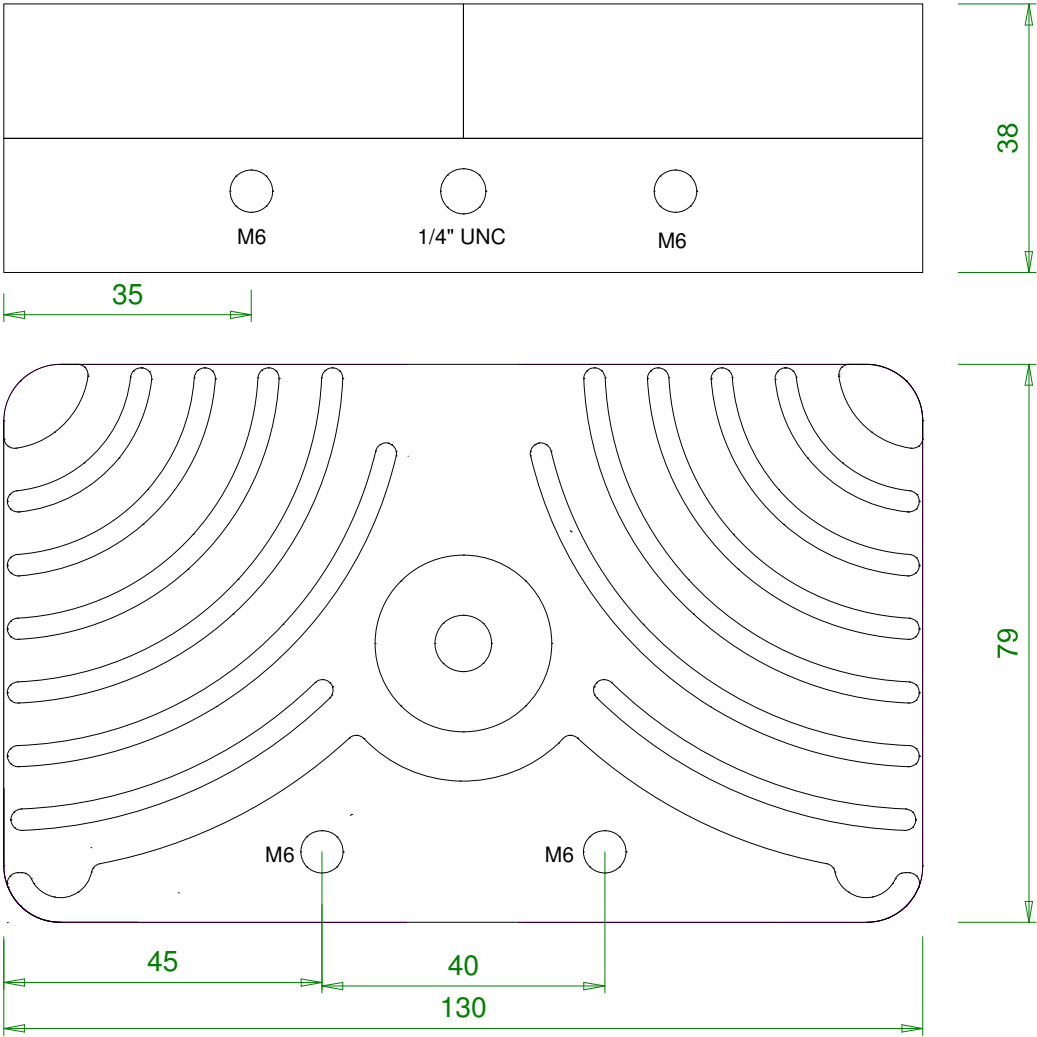
Mount plate for dual array
